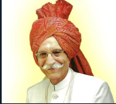
Source: StarsUnfolded
